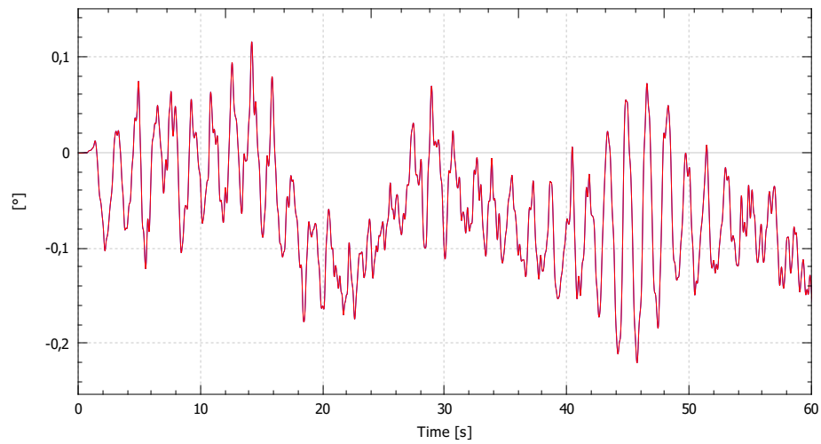
Yaw error
